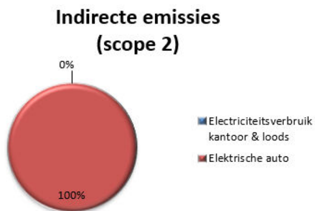
Figuur 4– Totale emissies scope 1 & 2 in ton CO 2
